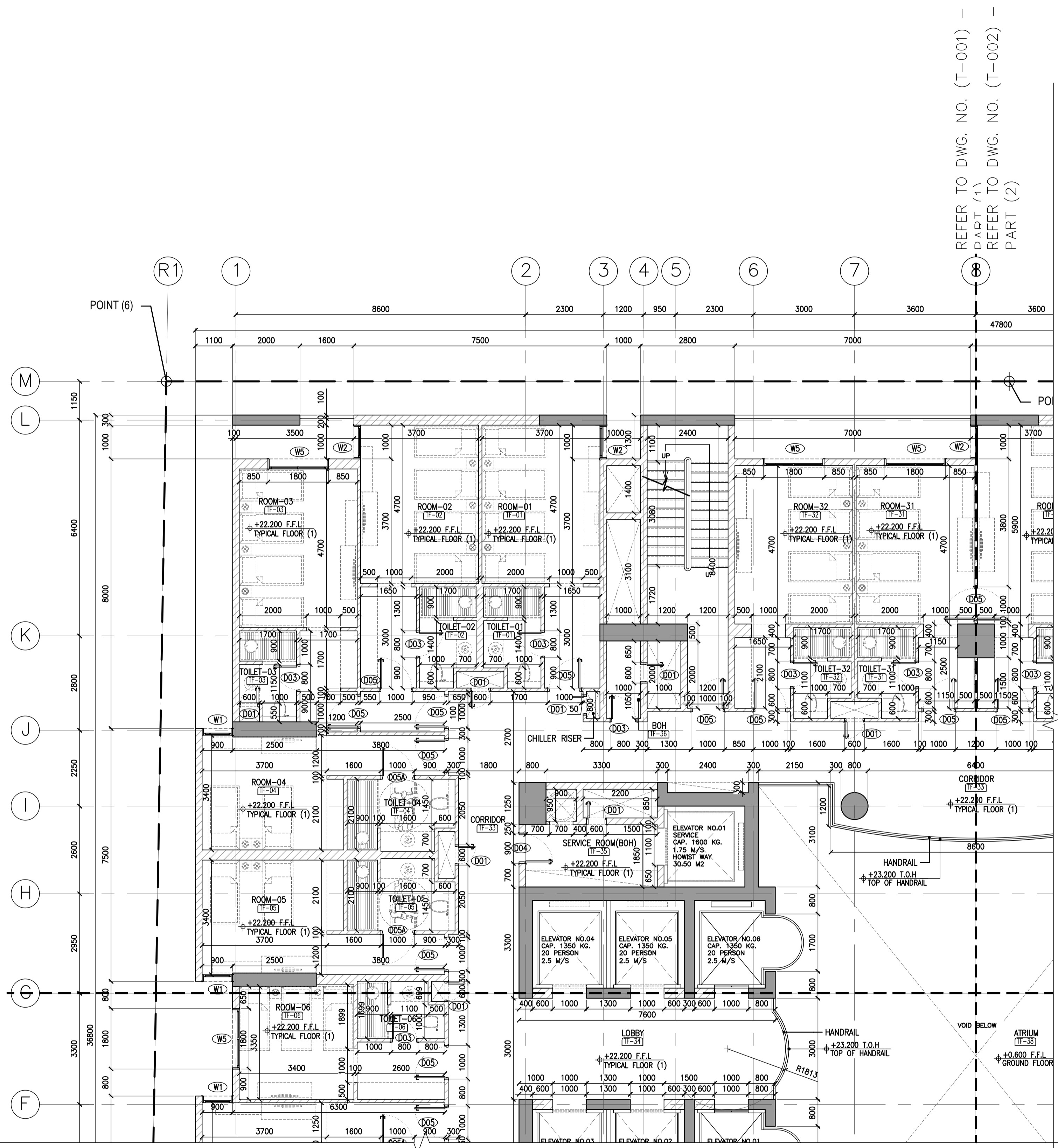
1 GENERAL PLAN - TYPICAL FLOOR - PART 1/4 SCALE 1:100
